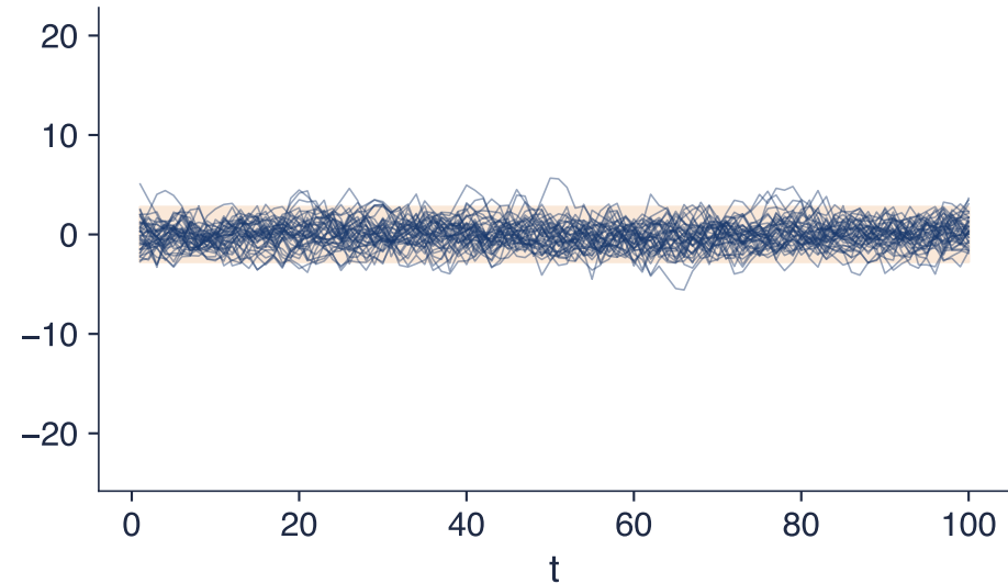
Stationary AR(1), \phi = 0.7 : same band at every t
