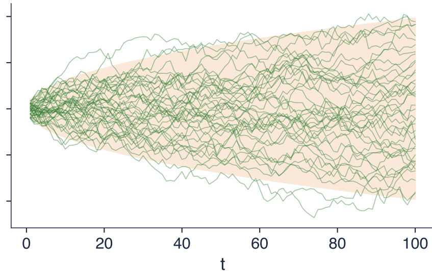
Random walk: the band widens like \sqrt{t}
