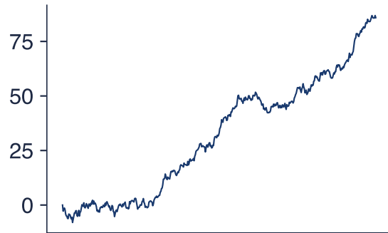
Series F
