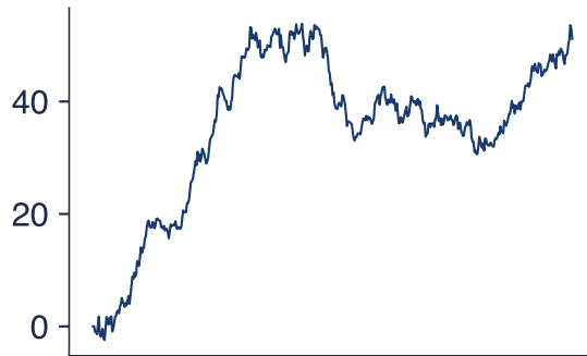
Series E
