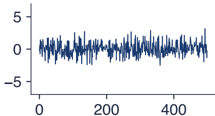
Gaussian i.i.d.
