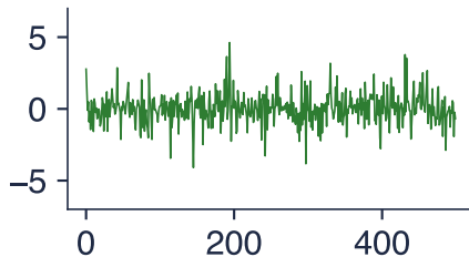
Laplace i.i.d.
