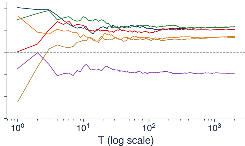
X_t = Z + \varepsilon_t : \bar{X}_T \rightarrow Z , not \mu = 0
