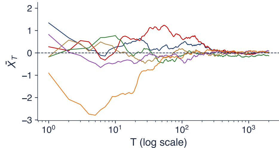
AR(1), \phi = 0.7 : \bar{X}_T \rightarrow \mu = 0 on every path
