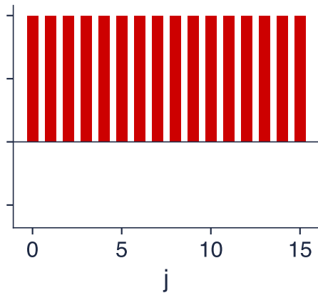
Random walk: \psi_j = 1 (no decay)
