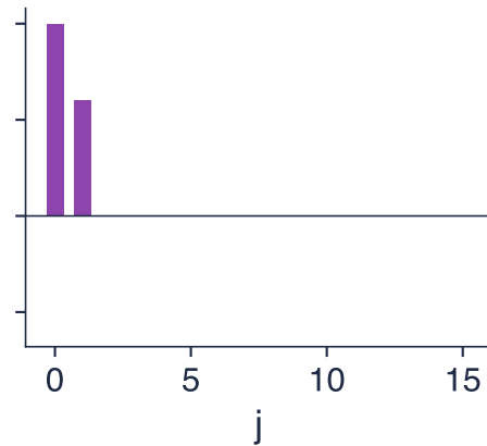
MA(1), \theta = 0.6 : \psi_1 = 0.6 , then 0
