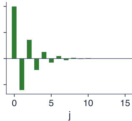
AR(1), \phi = -0.6 : \psi_j = (-0.6)^j
