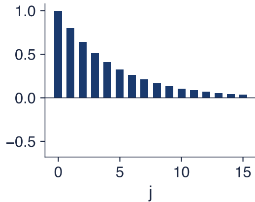
AR(1), \phi = 0.8 : \psi_j = 0.8^j
