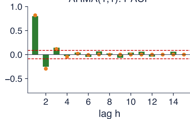
ARMA(1,1): PACF
