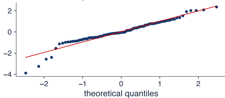
Normal QQ plot of the standardised residuals
