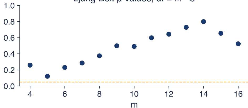
Ljung-Box p-values, df = m - 3
