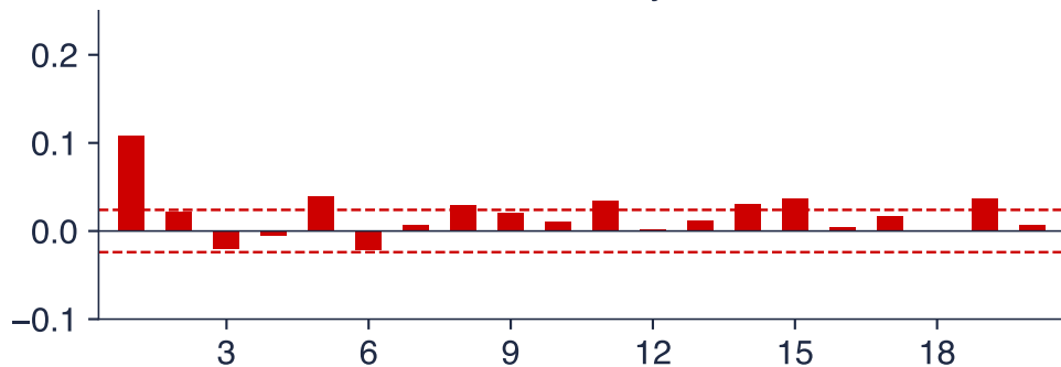
BET: ACF of daily returns
