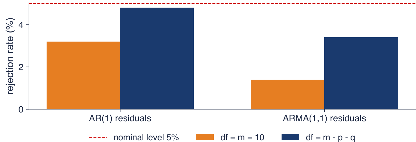
Ljung-Box on residuals of the true model, T = 200 , m = 10
