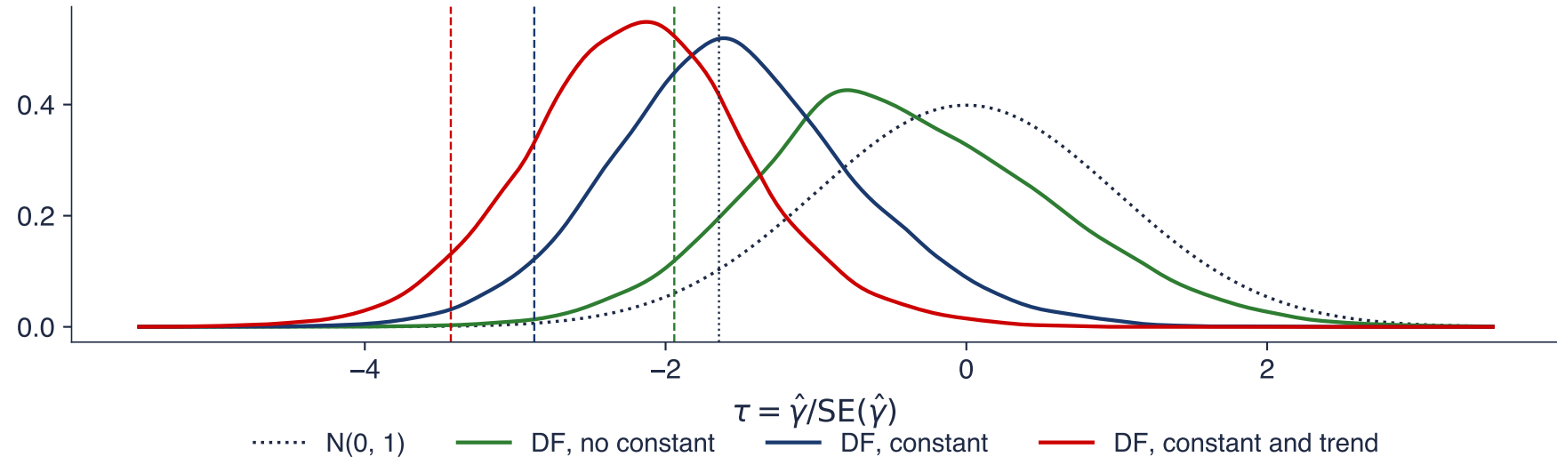
Null distribution of the Dickey-Fuller statistic (random walk, T = 250 ); dashed: 5% critical values
