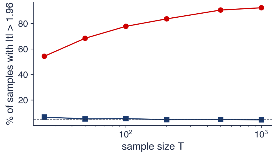
Rejection rate of a true null
