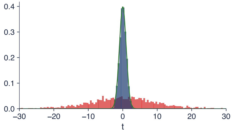
t-statistic of the slope, T = 200
