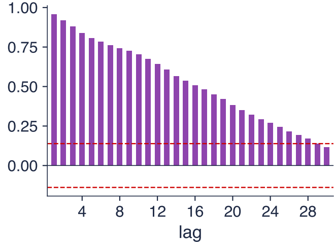
ACF of the residuals
