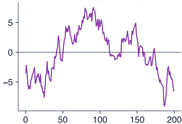
Residuals: apparent cycles
