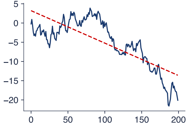
A driftless random walk and a fitted line
