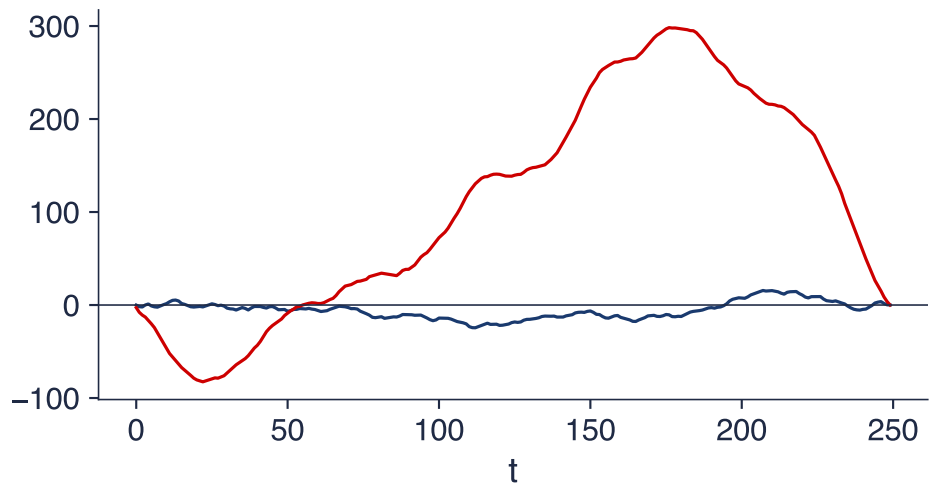
Partial sums S_t = e_1 + \dots + e_t
