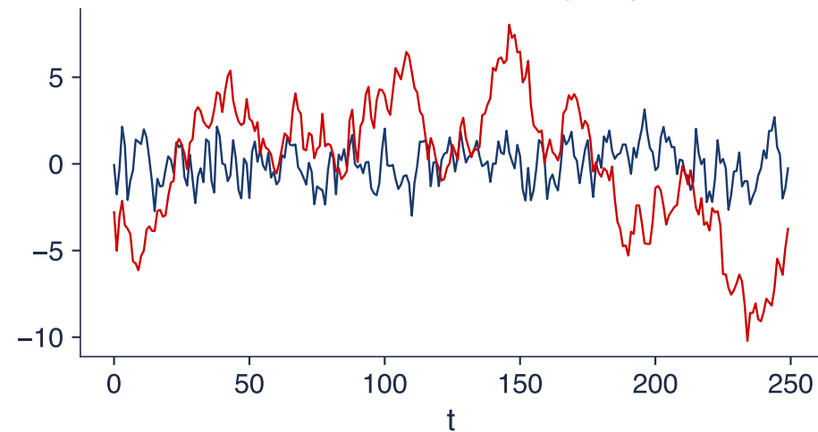
Demeaned series e_t = y_t - \bar{y}
