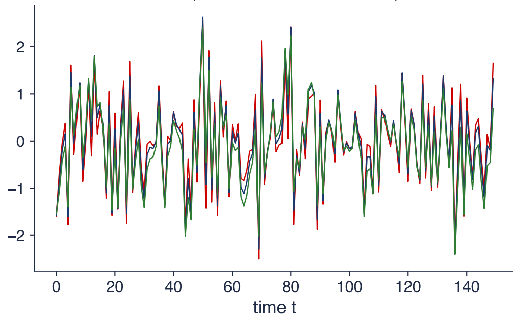
its increments (fractional Gaussian noise), first 150
