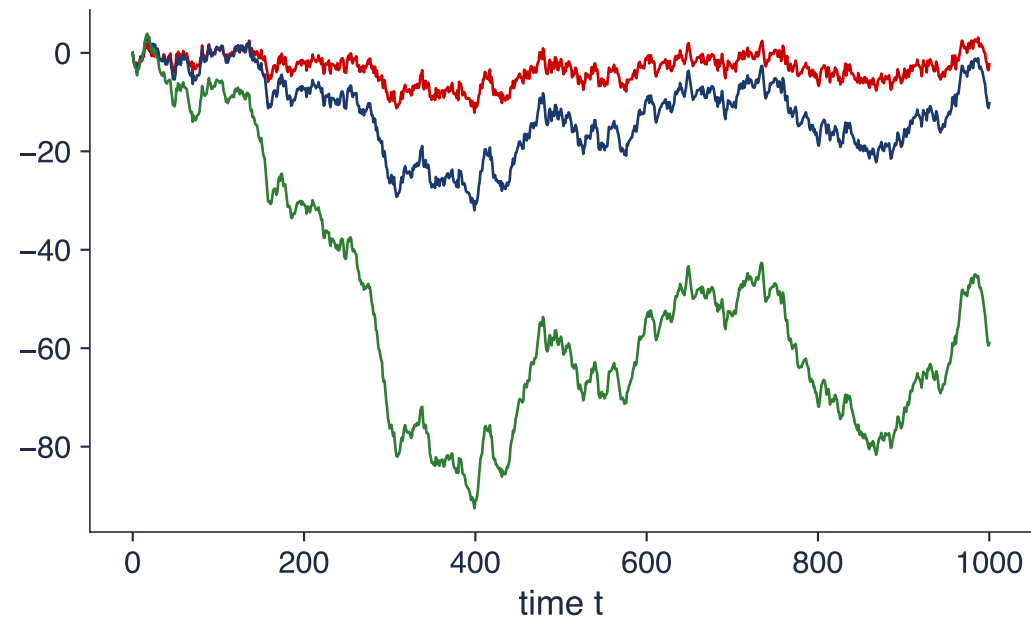
fractional Brownian motion B_H(t)
