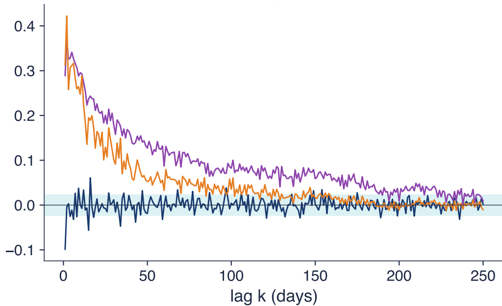
S&amp;P 500, daily, 2000-2026
