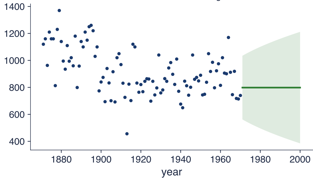
forecasts 1971-2000 as missing values
