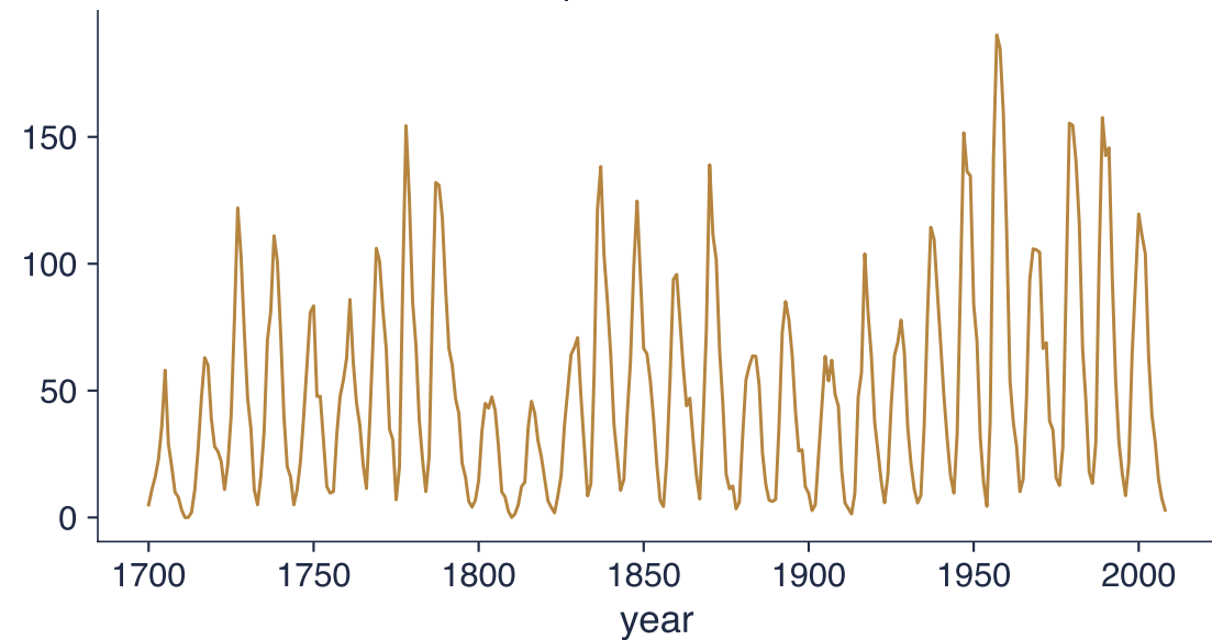
Sunspots, 1700-2008
