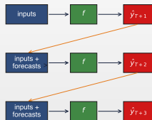
recursive: one model, applied 3 times
