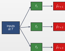
direct: one model per horizon
