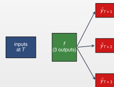
MIMO: one model, 3 outputs
