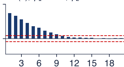
AR(2), \phi_1 = 0.5, \phi_2 = 0.3 : ACF
