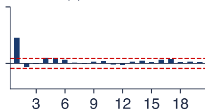
MA(1), \theta = 0.7 : ACF
