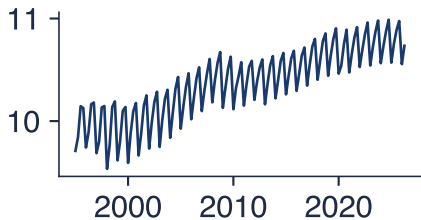
\ln Y_t
