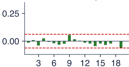
ACF of X_t^2
