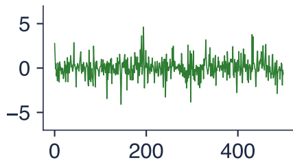
Laplace i.i.d.
