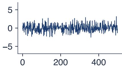
Gaussian i.i.d.
