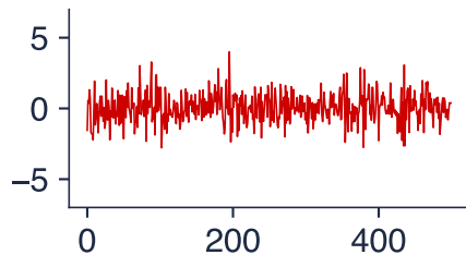
GARCH(1,1): weak WN
