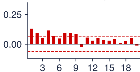
ACF of X_t^2
