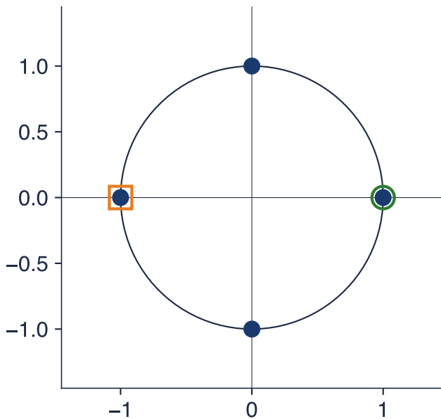
s = 4 : 4 roots of 1 - z^4
