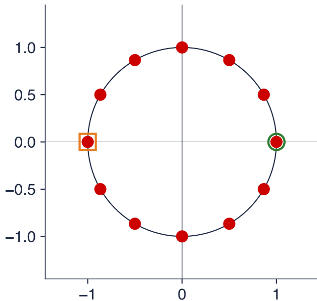
s = 12 : 12 roots of 1 - z^{12}
