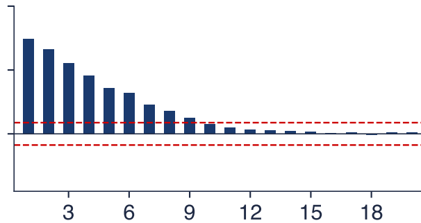
AR(2), \phi_1 = 0.5, \phi_2 = 0.3 : ACF
