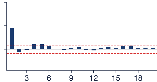
MA(1), \theta = 0.7 : ACF
