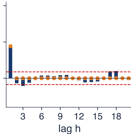
MA(1), \theta = 0.6
