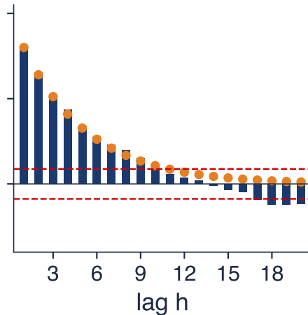
AR(1), \phi = 0.8
