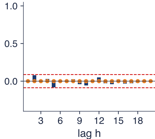
White noise
