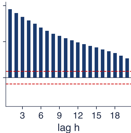
Random walk
