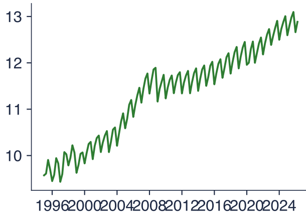
Box-Cox, \lambda = 0.02
