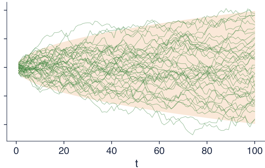
Random walk: the band widens like \sqrt{t}
