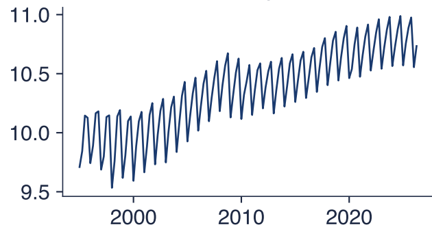
\ln Y_t
