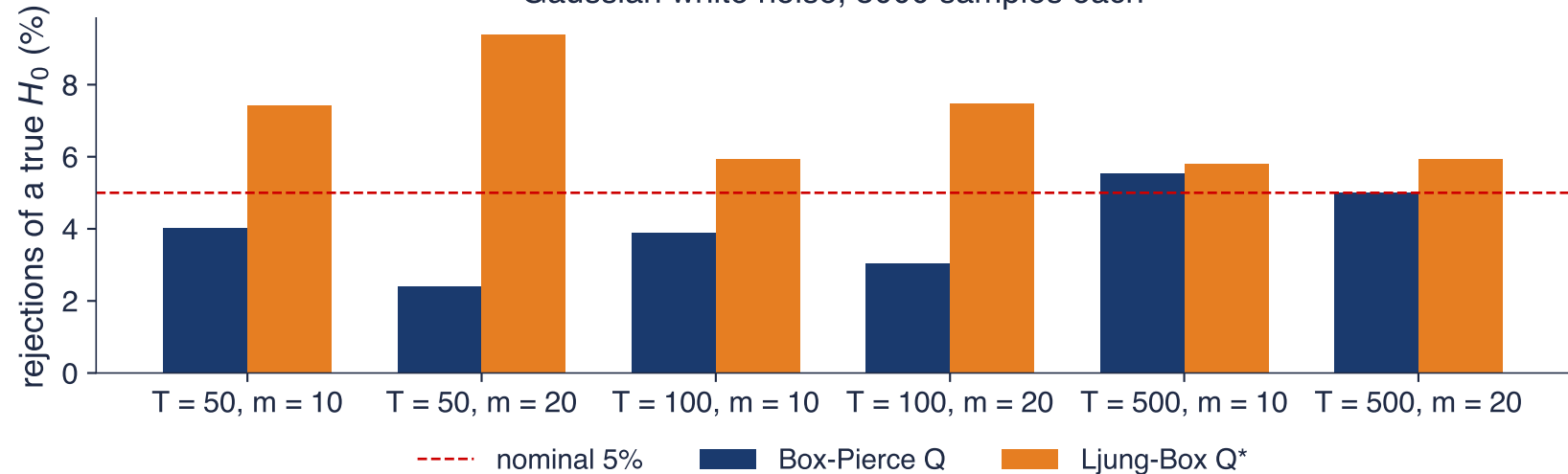
Gaussian white noise, 5000 samples each
