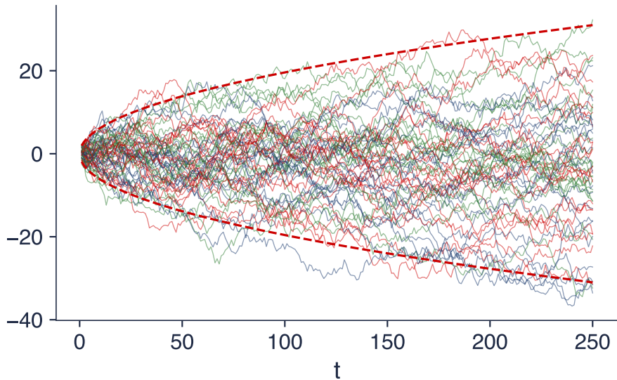
60 random walks, \sigma = 1
