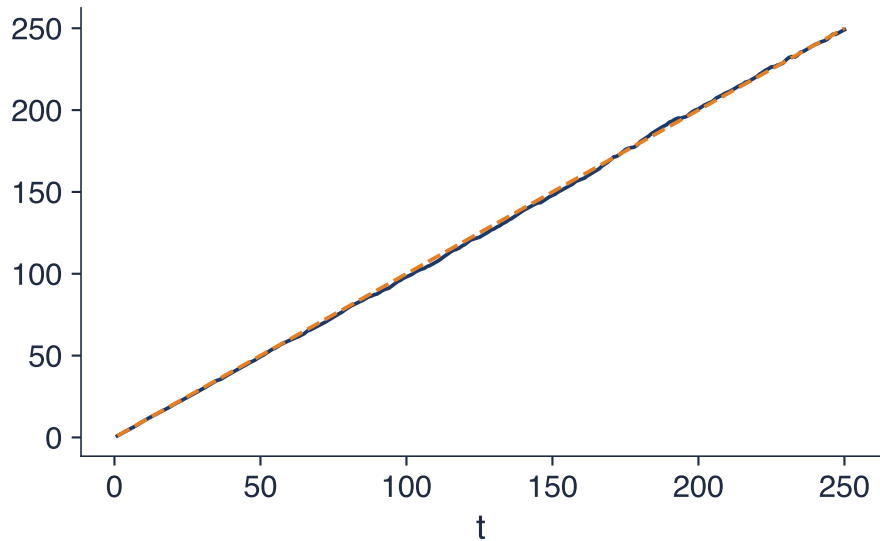
\text{Var}(X_t) grows linearly in t
