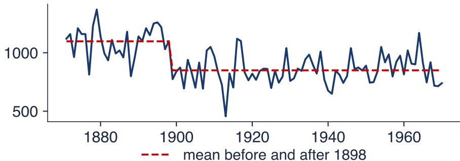
Nile at Aswan: yearly flow ( 10^8 \text{ m}^3 )
