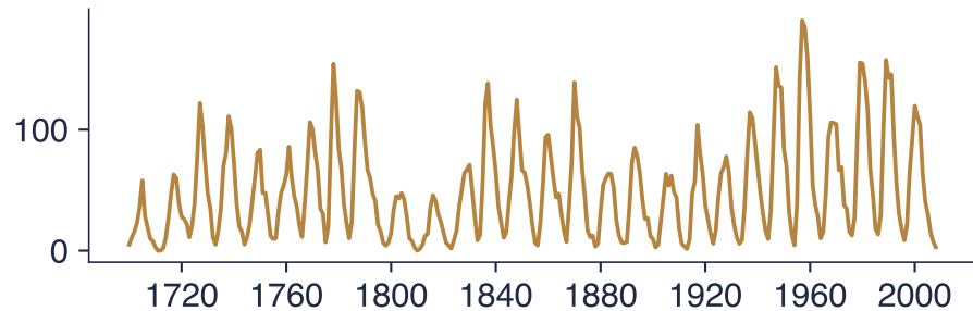
Yearly sunspot numbers
