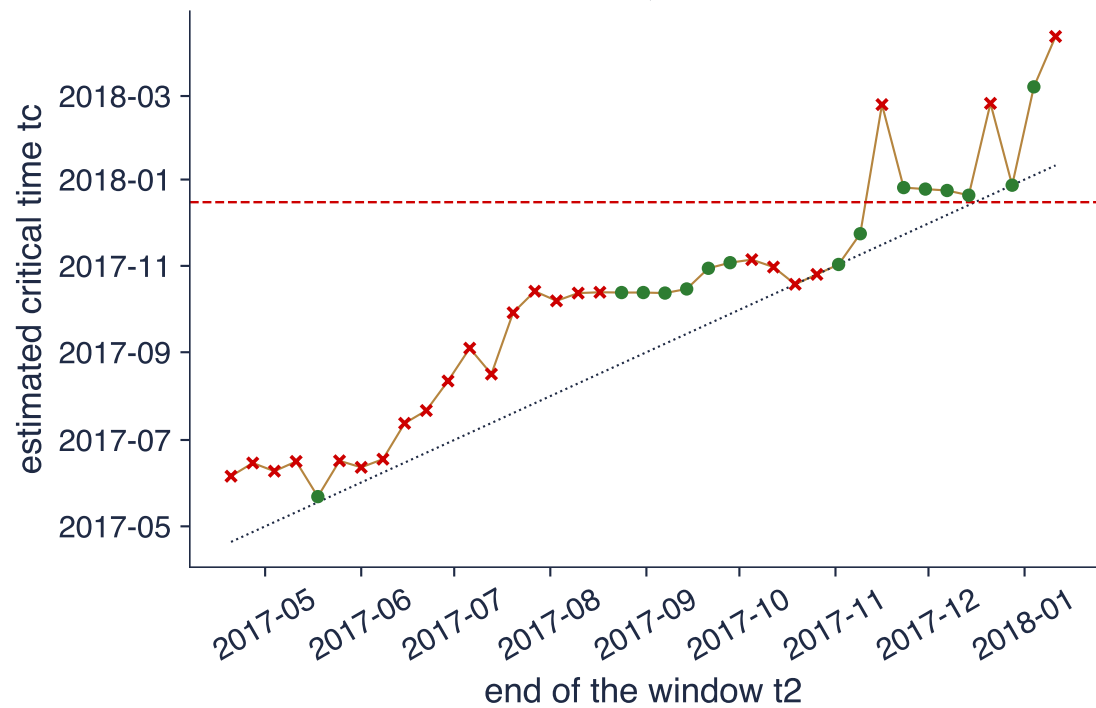
Bitcoin, 2017
