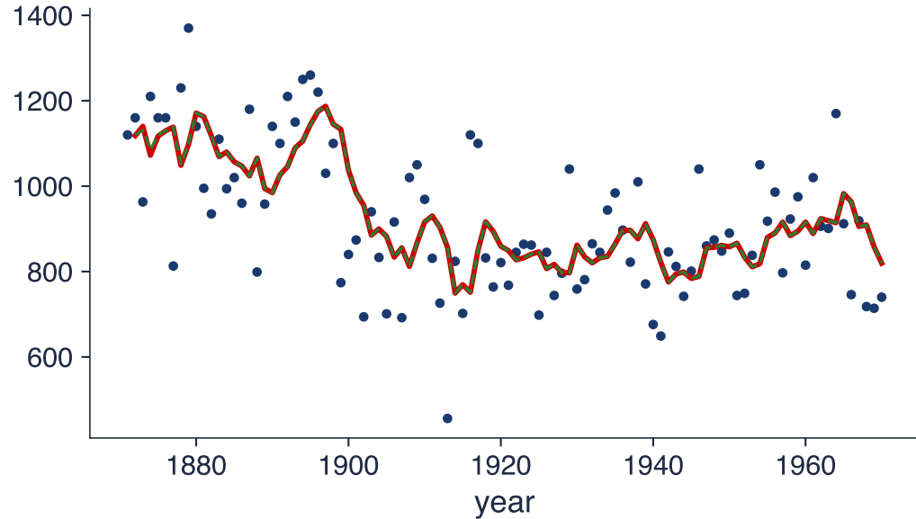
Kalman filter and exponential smoothing
