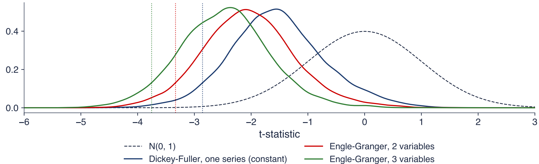
Null distributions of the t-statistic ( T = 200 , 10,000 simulations); dotted: 5% quantiles
