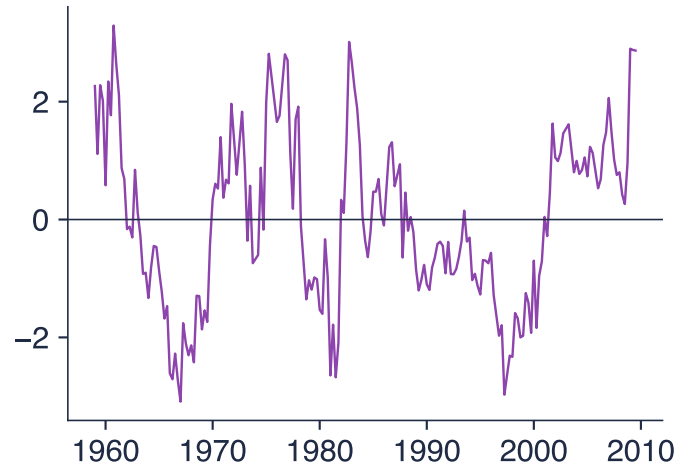
Consumption on income: residuals
