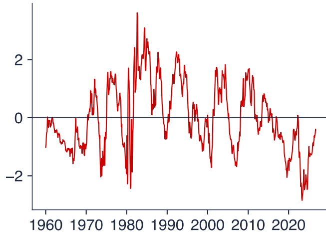
10-year on 3-month yield: residuals
