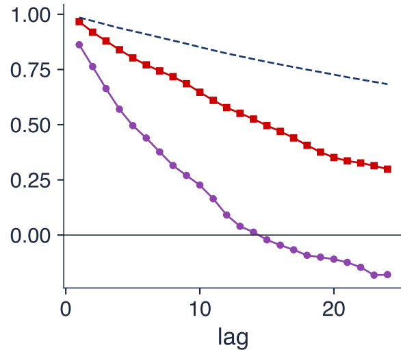
Sample ACF
