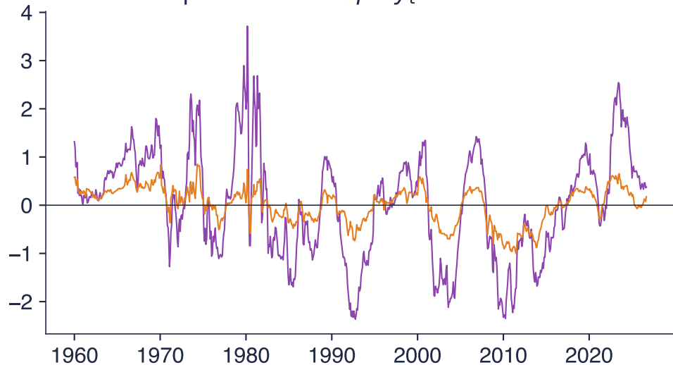
Equilibrium errors \hat{\beta}^\top y_t of the VECM
