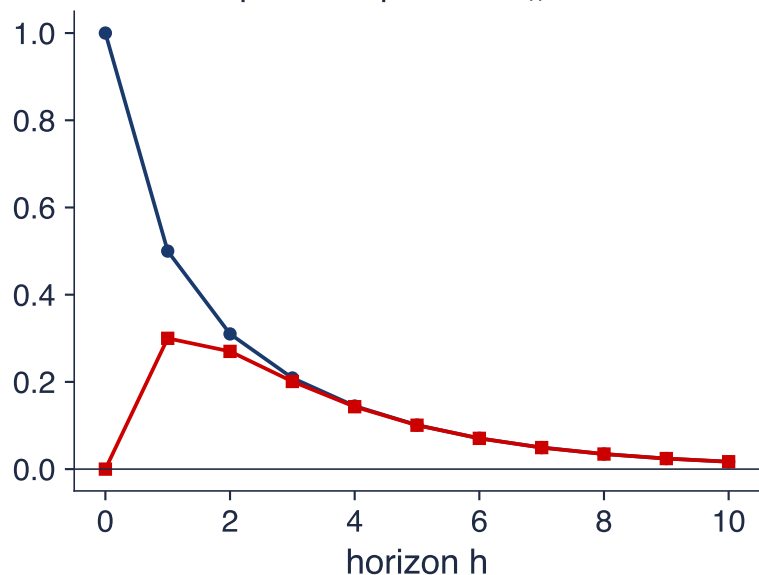
Impulse responses \Phi_h = A^h
