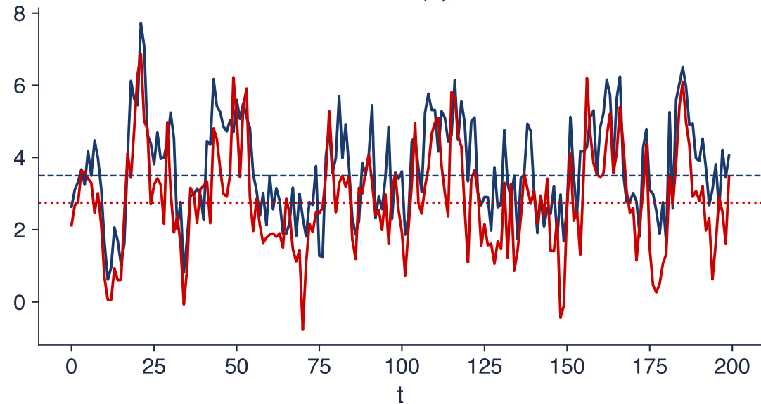
Simulated VAR(1), T = 200
