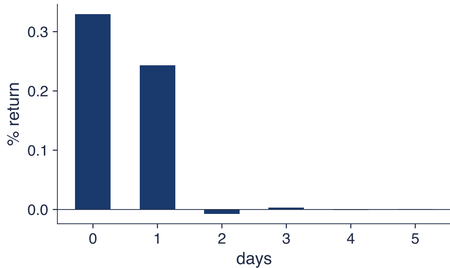
Generalised impulse response, VAR(1)
