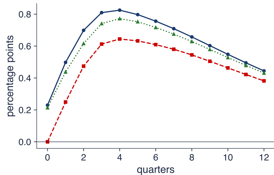
ROBOR 3M &lt;- inflation shock
