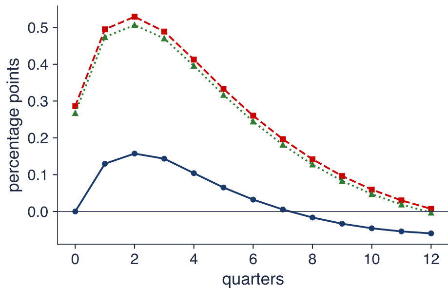
inflation &lt;- ROBOR 3M shock
