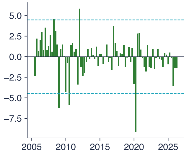
GDP growth equation
