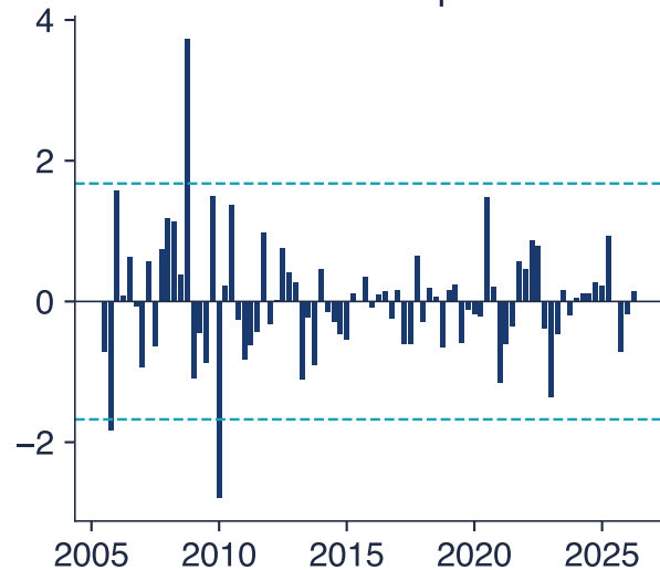
ROBOR 3M equation
