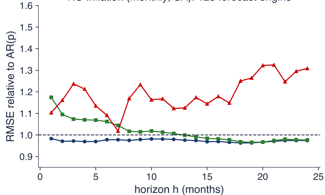
RO inflation (monthly, SA): 128 forecast origins
