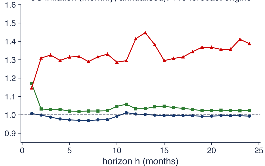
US inflation (monthly, annualised): 415 forecast origins
