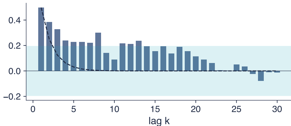
Nile flow
