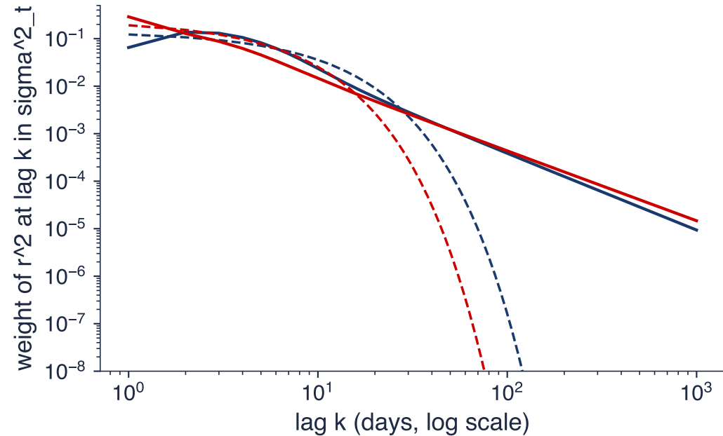
ARCH(infinity) weights
