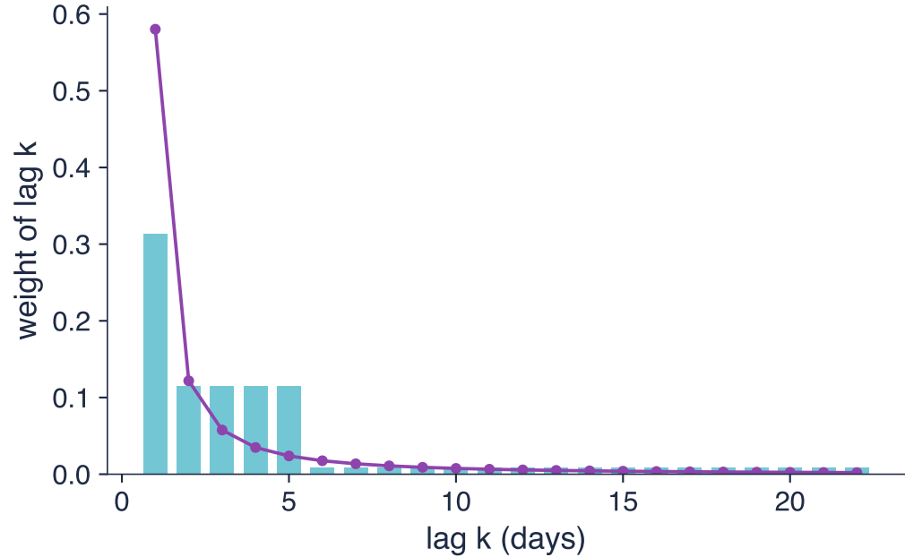
HAR: three steps that mimic a power law
