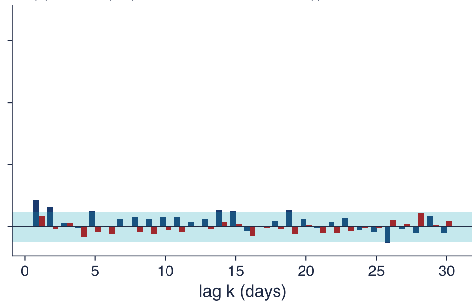
AR(1)-GARCH(1,1)-t: standardised residuals z(t)
