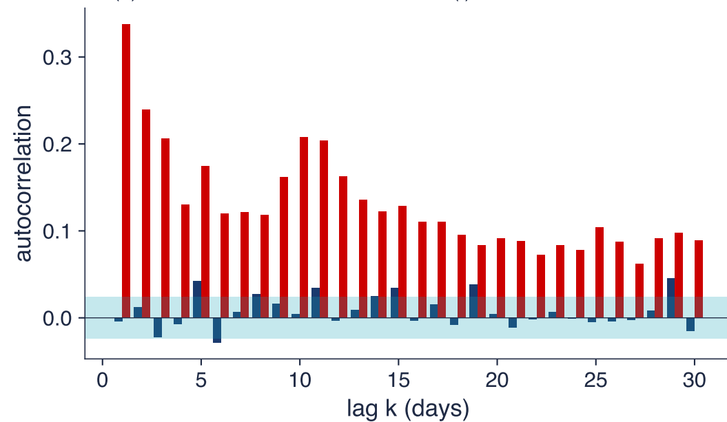
AR(1) with constant variance: residuals e(t)
