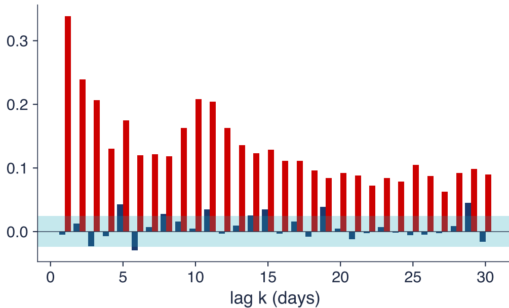
AR(1) with constant variance: residuals e(t)
