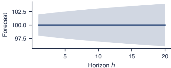
ARIMA(0,1,1), \theta = -0.6 : keeps widening
