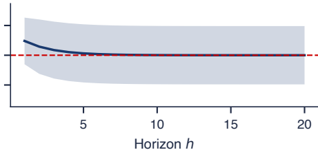
AR(1), \phi = 0.6 : bounded, back to the mean
