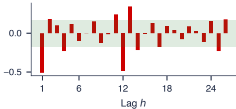
After both differences: spikes at lags 1 and 12
