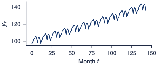
A monthly series ( s = 12 )
