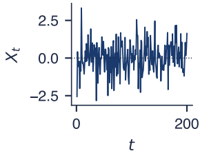
White noise
