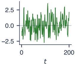
MA(1), \theta = 0.8
