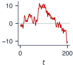
Random walk
