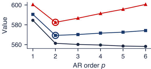
Simulated AR(2), T = 200
