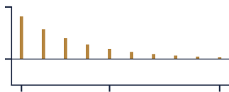
ARMA(1,1): PACF
