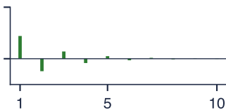
MA(1): PACF
