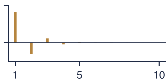
ARMA(1,1): PACF
