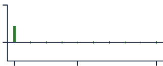
MA(1): PACF
