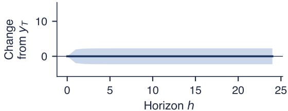
Stationary AR(1), \phi = 0.5 ( d = 0 )
