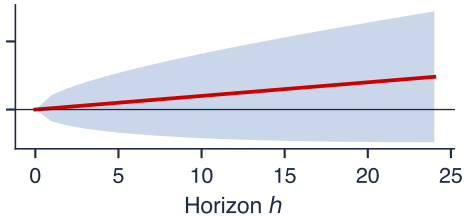
Random walk with drift 0.2 ( d = 1 )
